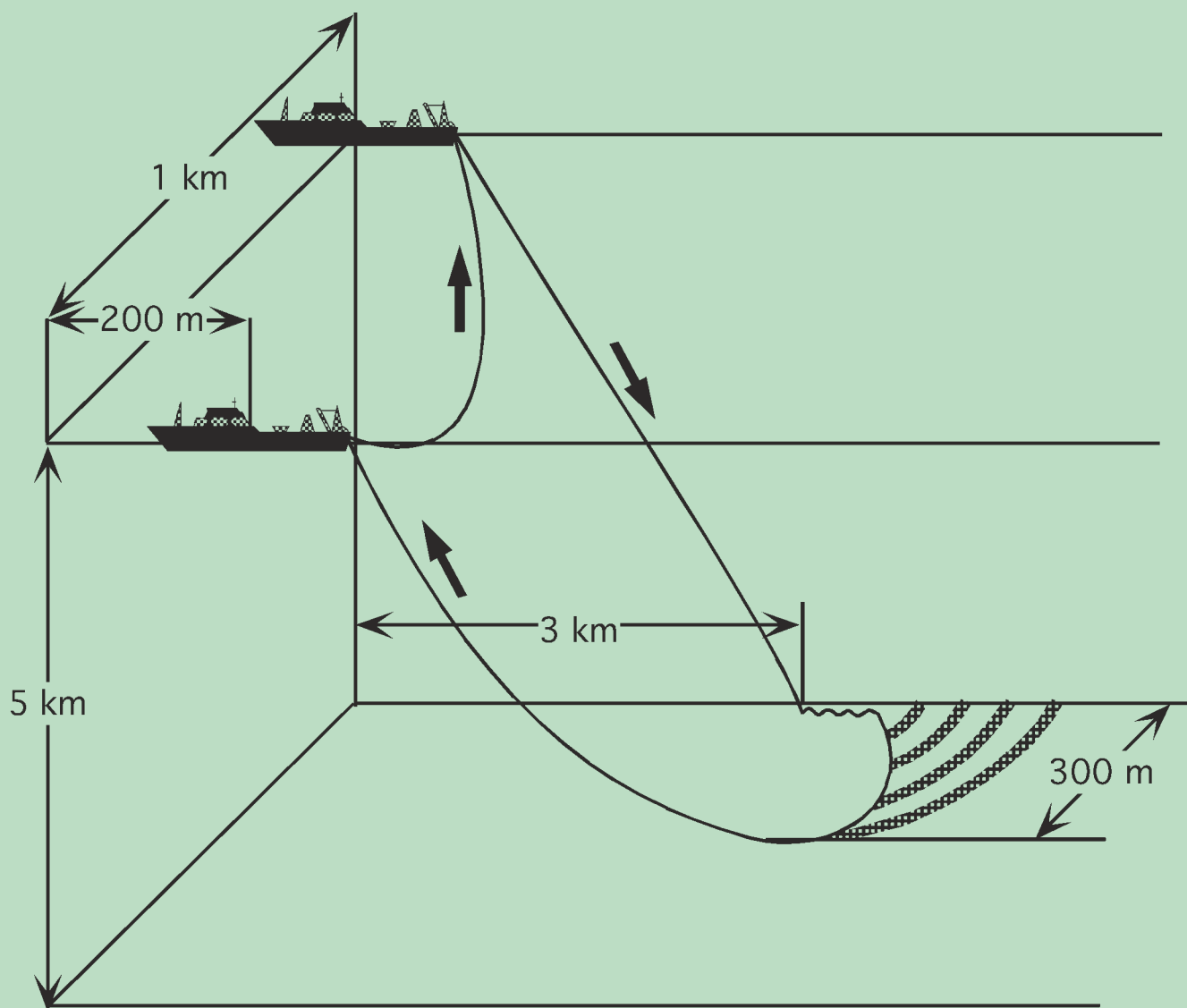
THE CLB SYSTEM (Continuous Line Bucket) with two vessels
