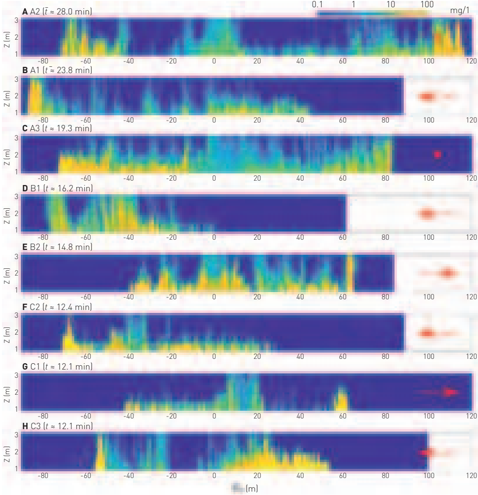
Figure 5.5: Data sets for the eight selfies conducted by Patania II. They show vertical profiles of sediment concentration detected by the instrumentation mounted on the vehicle as it drove through the sediment plume it had created. The red arrows on each plot indicate the direction of the background ocean current; a red dot represents no significant current. The location X = 0 corresponds to the location of the track where Patania II had created the sediment plume a few minutes earlier.
