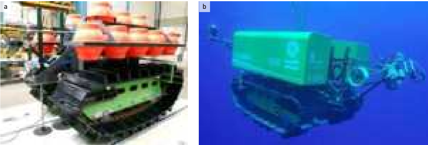
Figure 3.3: (a) Construction and (b) deployment of the Patania I concept vehicle for testing trafficability during the GSRNOD17 campaign. The circular pressure-sinkage plate can be seen mounted at the front of the vehicle in (a).
