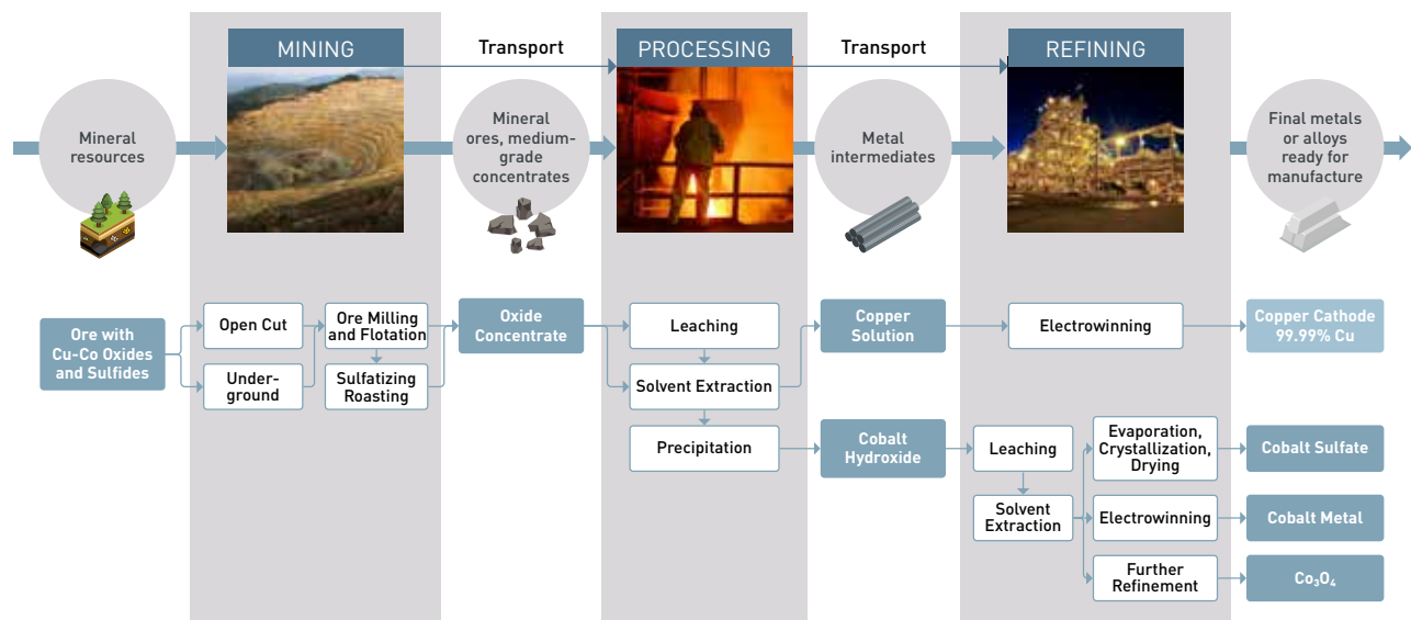
Figure 24. Cobalt Production as Byproduct of Copper Oxides (Hydro) 121
