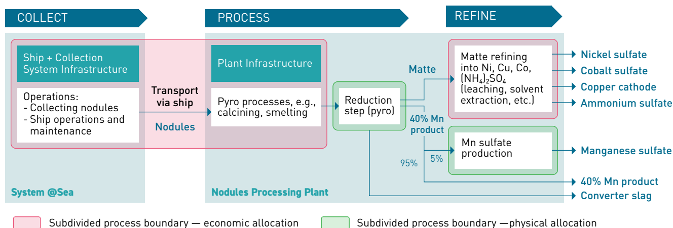
Figure 19. Nodule Operations Impact Allocation Design Block Diagram 88
