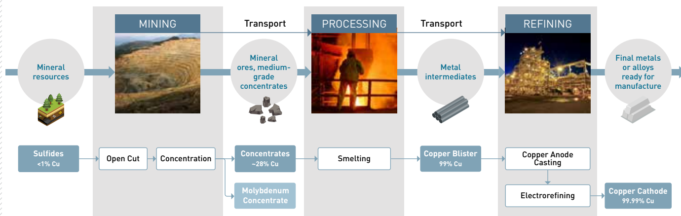
Figure 26. Copper Production from Sulfides (Pyro)
