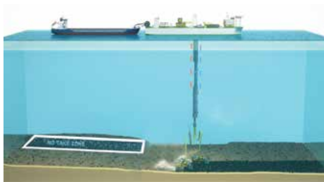
b) Deep-sea nodules collector concept
