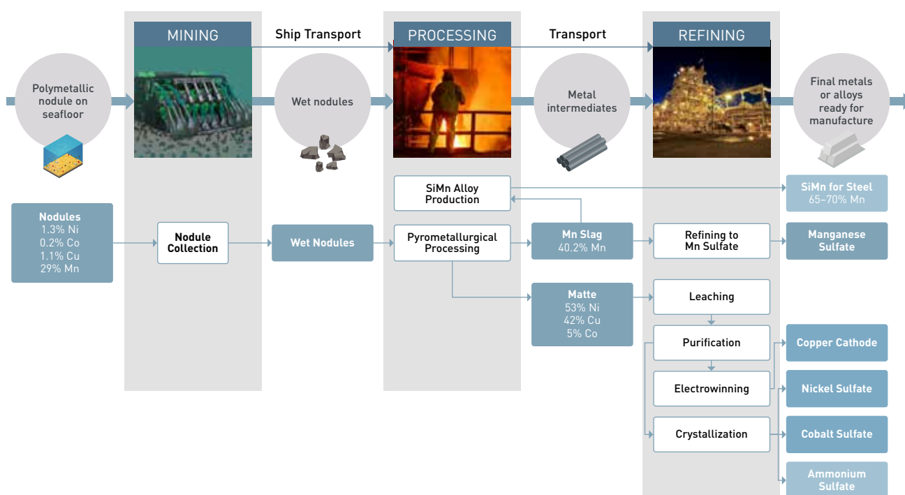
Figure 30. Processing Polymetallic Deep-Sea Nodules
