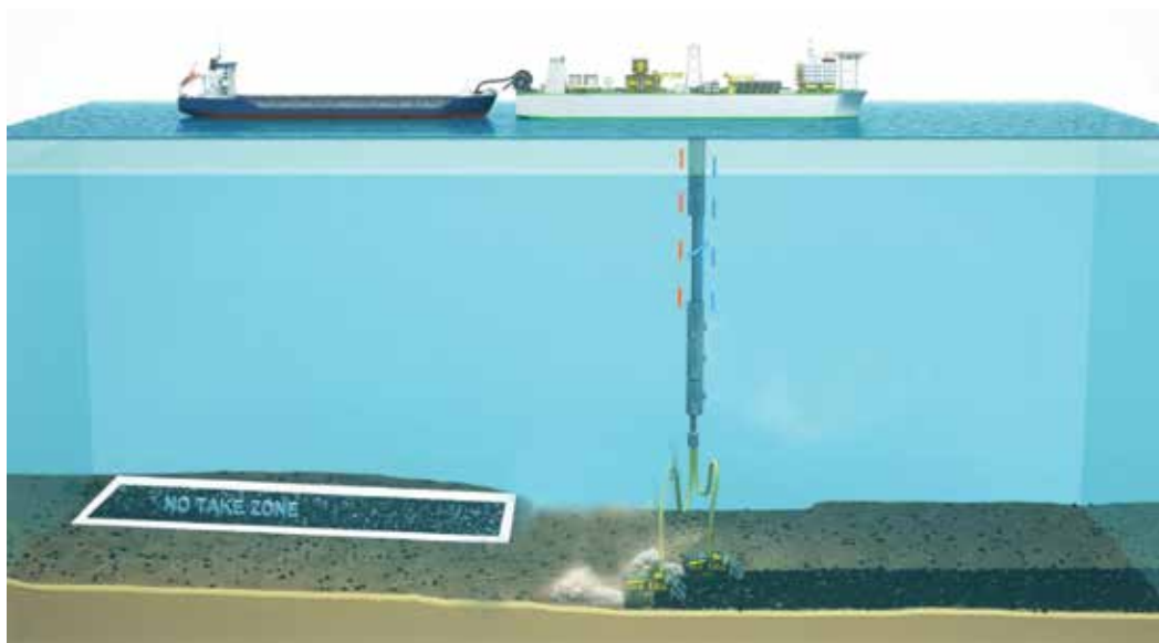
Figure 29. Nodule Collection System Including Production Vessel and Riser
