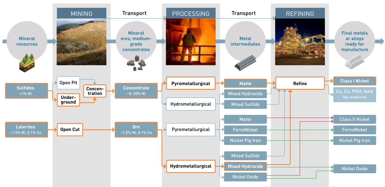
Figure 23. Several Production Paths for Nickel from Land Ores (Two Typical Class I Paths Highlighted)
