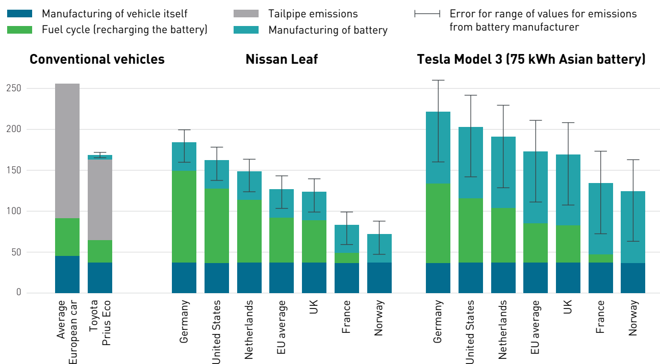
Figure 10. Life Cycle GHG Emissions (CO 2 e Grams per Kilometer) 45
