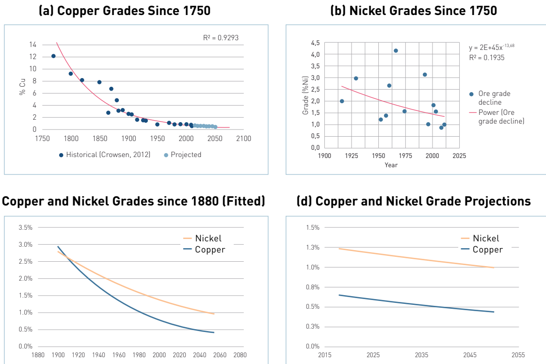
Figure 42. Historical and Fitted Copper and Nickel Ore Grades (Sulfides and Laterites) 160
