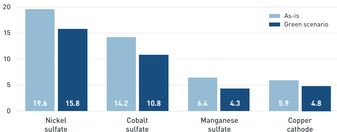
Figure 45. Per-kg CO 2 e for Land Ores (kg), Comparing As-Is (2017) to Green Scenario (2047)
