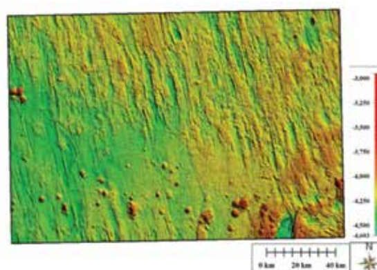
Figure 59. Sample Seafloor Topography in the CCZ 246
