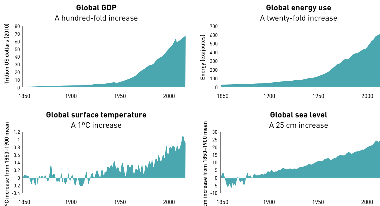
Figure 2. Human Activity, Global Surface Temperatures, and Sea-Level Increase 17
