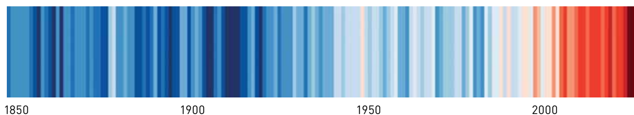
Figure 3. Annual Global Temperatures, 1850–2017 18
