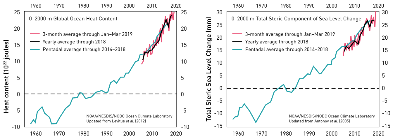
Figure 5. Global Ocean Heat Content (Left) and Total Steric Sea-Level Anomaly (Right) 23
