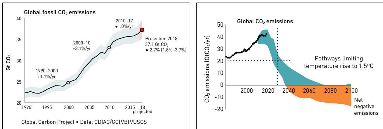
Figure 7. Global CO 2 Emissions from Human Activity (L); Emissions Pathway to Limit Rise to 1.5°C (R) 32
