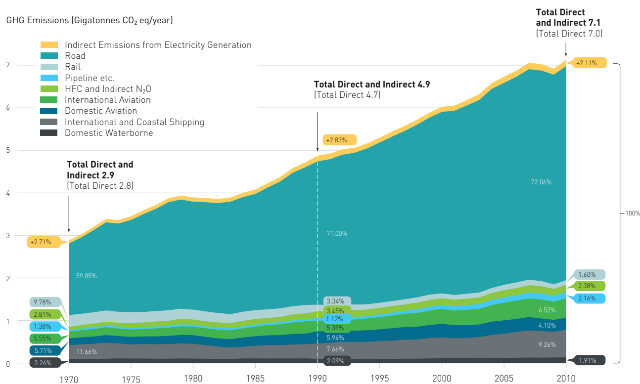
Figure 8. GHG Emissions from Transport, 1970–2010 (Gigatonnes CO 2 Equivalent/Year) 36
