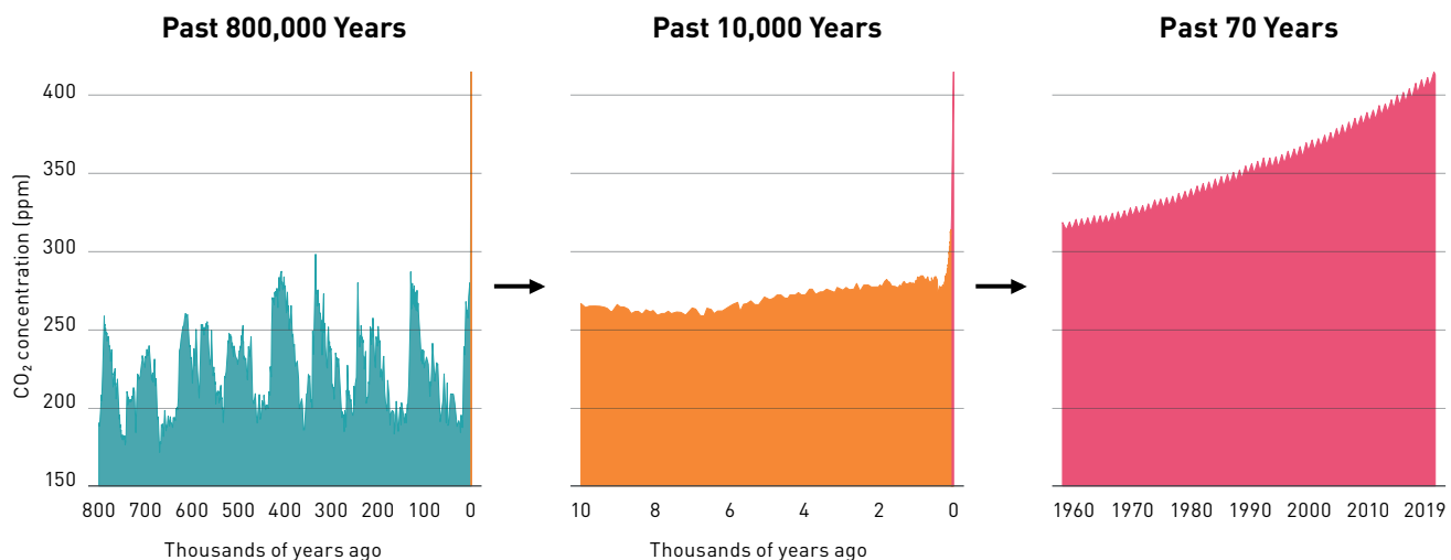
Figure 1. Atmospheric CO 2 Concentration: Historical Through August 13, 2019 (parts per million) 15
